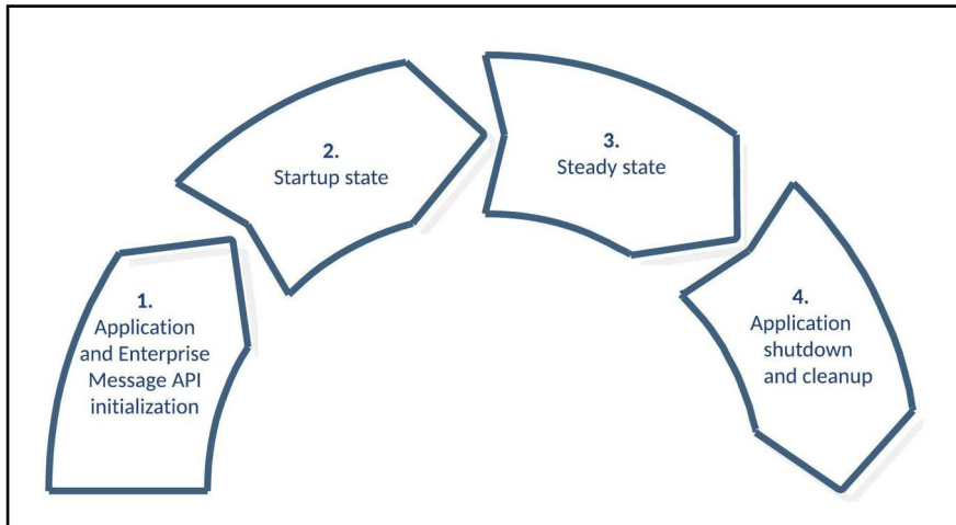
Figure 10. EmaCppConsPerf Lifecycle
