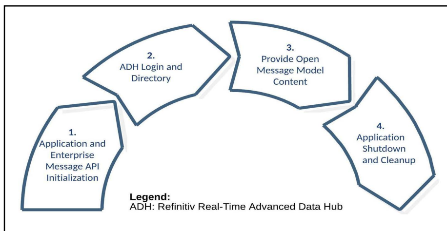
Figure 14. EmaCppNIProvPerf Lifecycle
