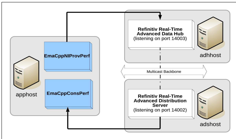
Figure 18. EmaCppNIPProvPerf to Consumer on the Refinitiv Real-Time Distribution System
