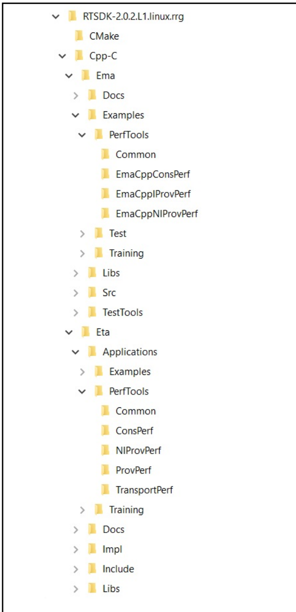
Figure 4. Directory Structure of the Performance Tools
