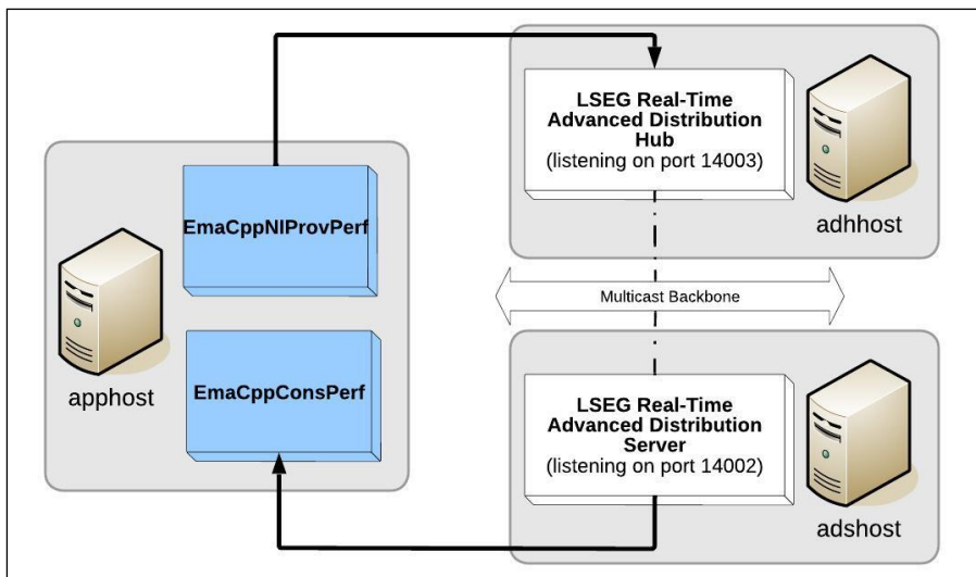
Figure 17. EmaCppNIProvPerf to Consumer on the LSEG Real-Time Distribution System
